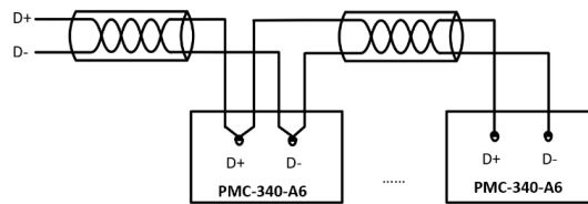
Figure 2-7 RS-485 Wiring
