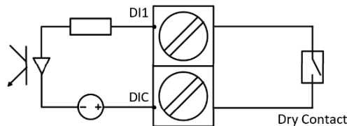
Figure 2-8 Digital Input
