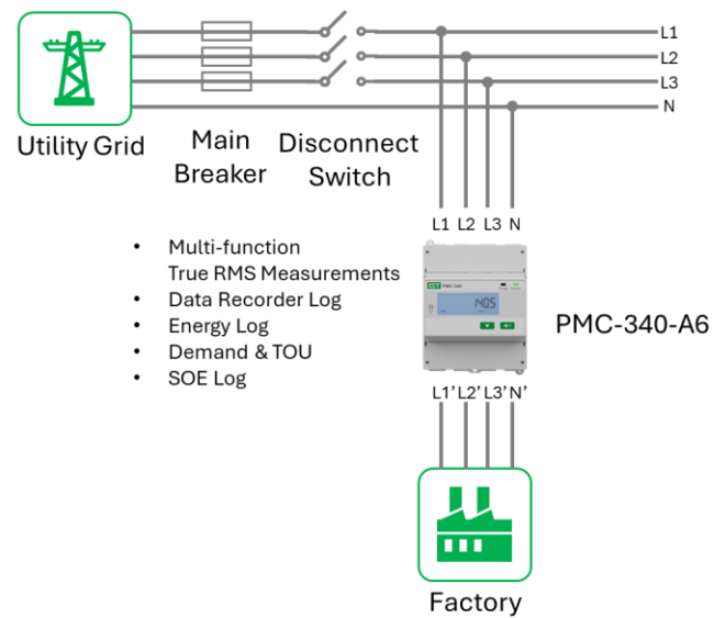
Figure 1-1 Typical Application
