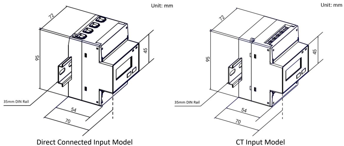
Figure 2-4 Installations
