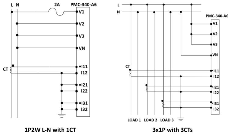
Figure 2-6 CT Input Wiring Connection
