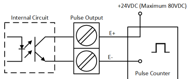
Figure 2-9 Solid State Relay Connections for Energy Pulsing
