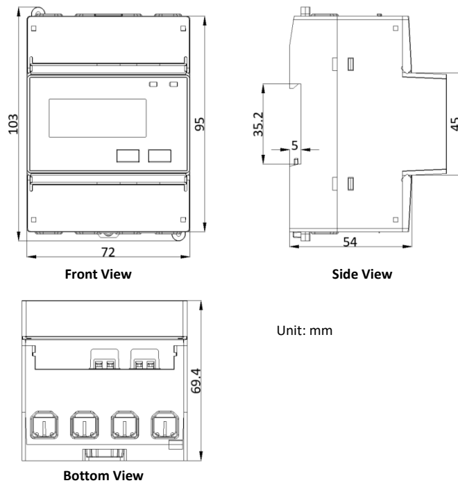
Figure 2-3 Unit Dimensions
