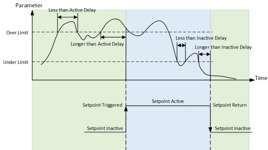
Figure 4-1 Over Setpoint
