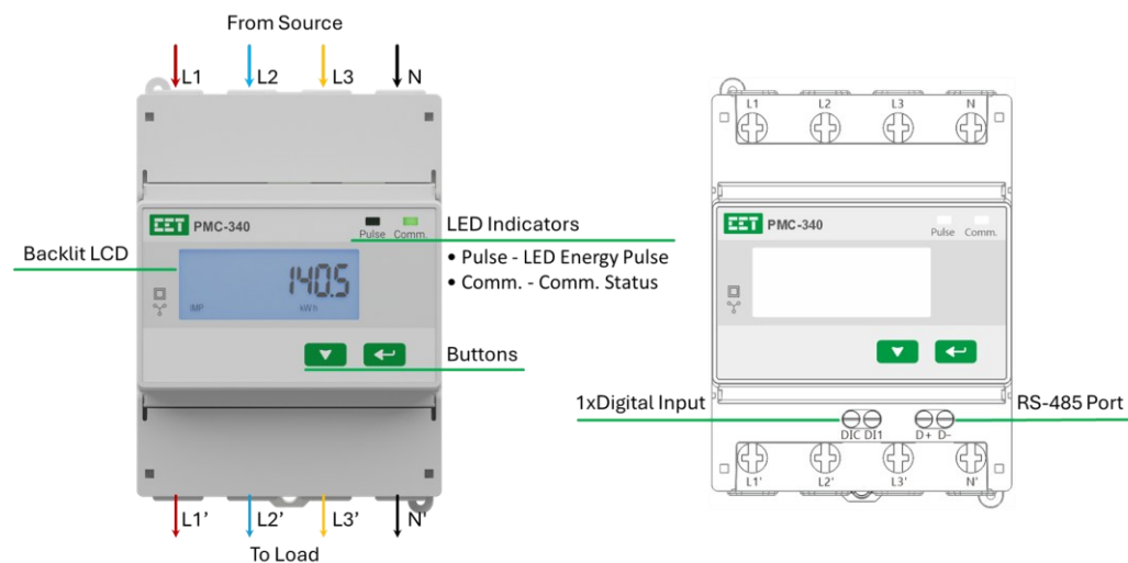
Direct Connected Input Model with I/O Option B
