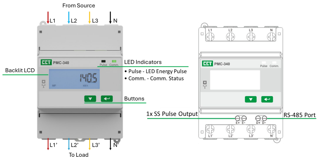
Direct Connected Input Model with I/O Option A
