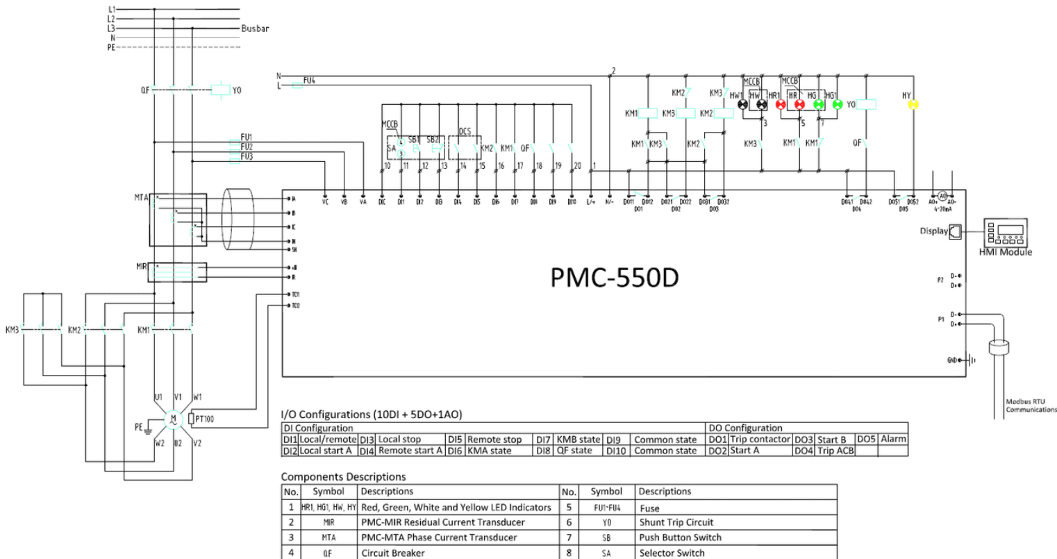
Figure 2-38 Star-Delta Start Schematic Diagram
