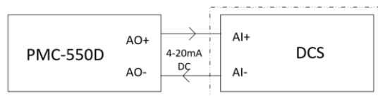
Figure 2-33 Analog Output Wiring
