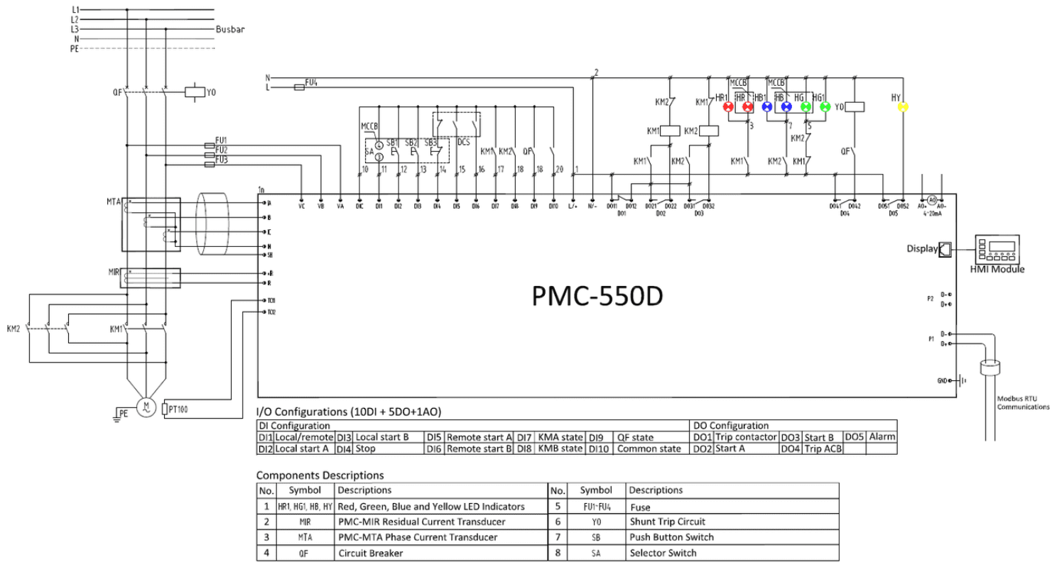
Figure 2-41 Forward-reverse Operation Schematic Diagram
