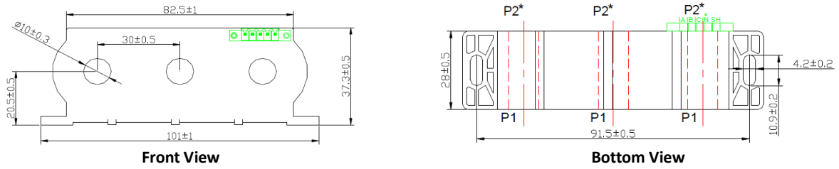
Figure 2-13 PMC-MTA-1A / PMC-MTA-5A Dimensions
