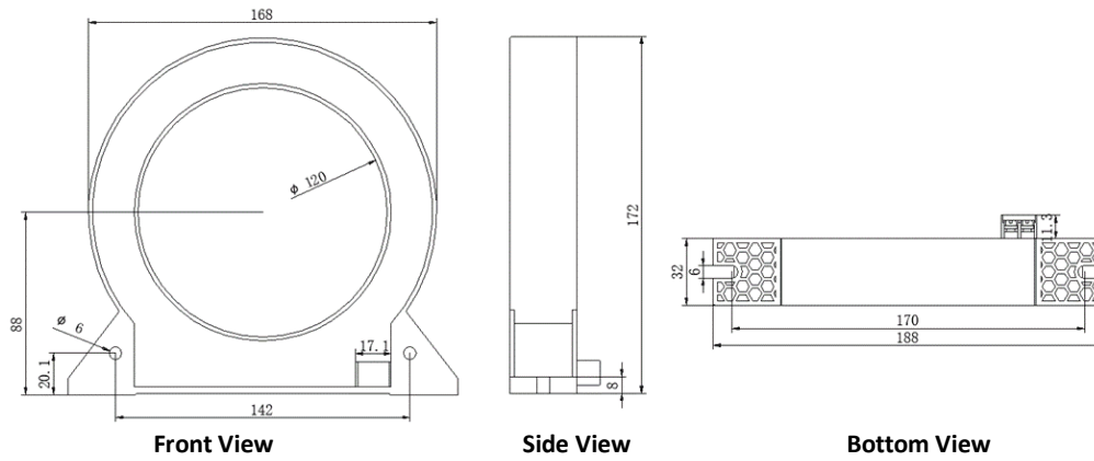
Figure 2-21 PMC-MIR-120 Dimensions
