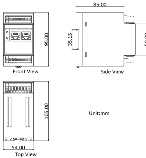
Figure 2-12 Expansion Module's Dimensions
