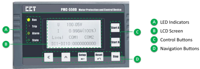
Figure 2-3 HMI Display Module
