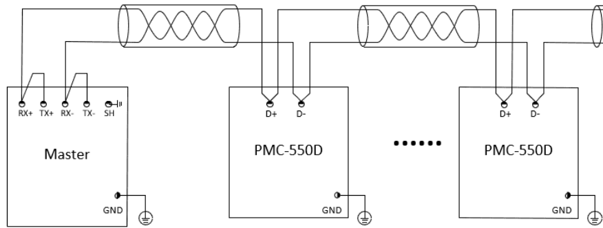
Figure 2-34 Wiring Diagram of RS-485 Communication
