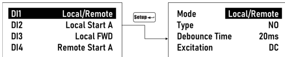
Figure 3-23 Digital Inputs Setup Screens
