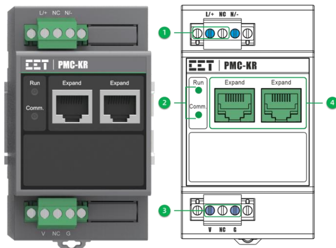
Figure 2-5 PMC-KR Front View and Terminals Diagram
