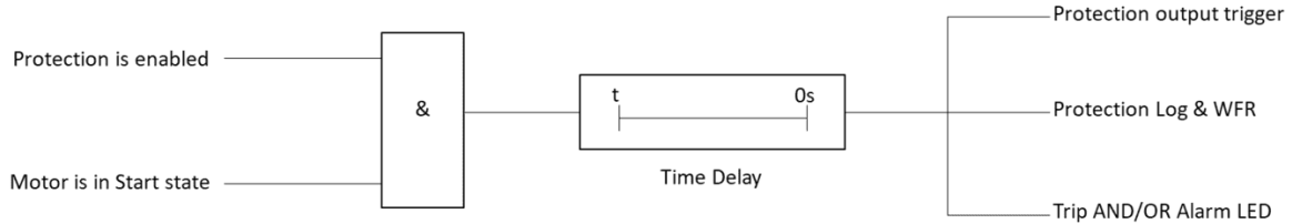
Figure 4-2 Logic Diagram of Long Start Protection
