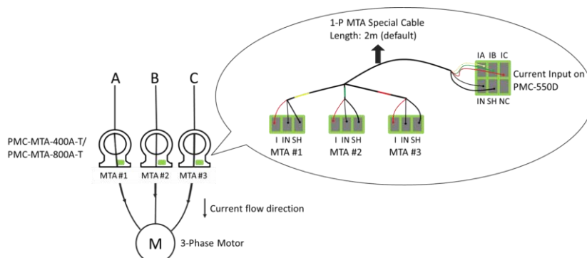
Figure 2-30 PMC-MTA-400A-T / PMC-MTA-800A-T Connections
