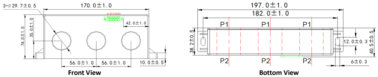
Figure 2-15 PMC-MTA-100A / PMC-MTA-300A Dimensions
