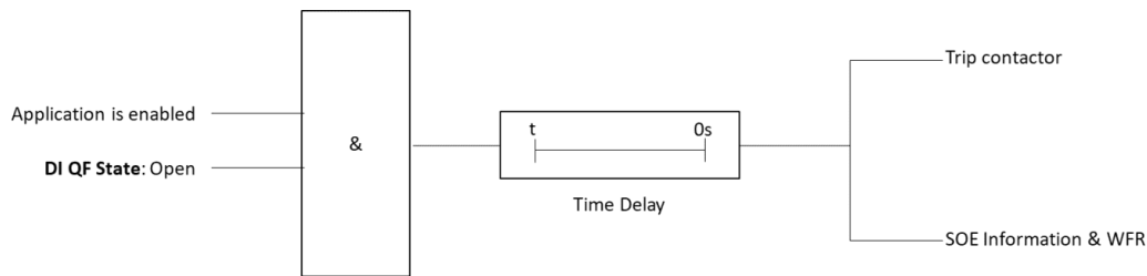
Figure 4-16 ACB Control Contactor Application Logic Diagram
