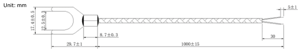
Figure 2-25 NTC-Y12 Dimensions
