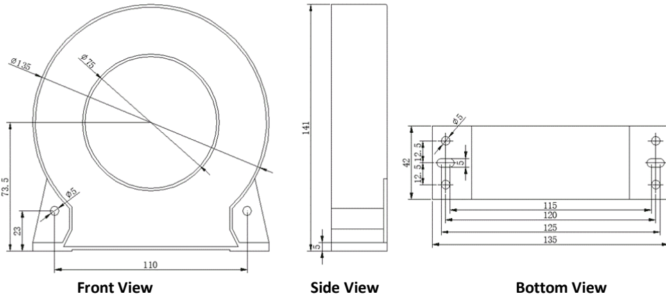
Figure 2-20 PMC-MIR-75 Dimensions
