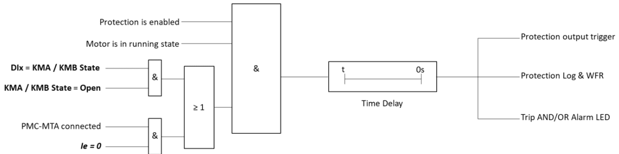
Figure 3-17 Logic Diagram of CB Failure Protection
