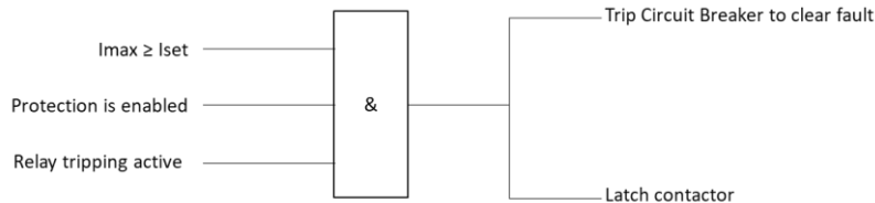
Figure 3-18 Logic Diagram of Contactor Protection
