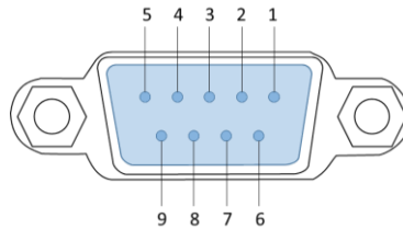
Figure 2-35 PROFIBUS DP DB9 Pinout
