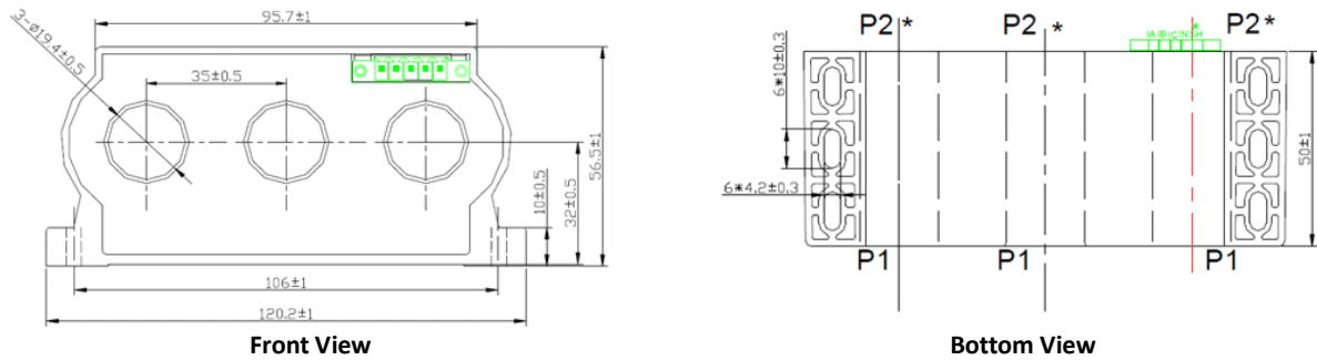
Figure 2-14 PMC-MTA-25A Dimensions
