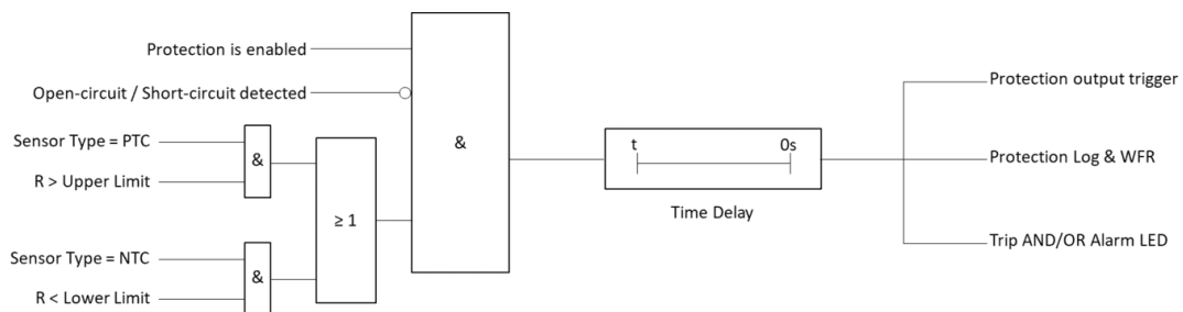
Figure 4-18 Logic Diagram of Thermo Resistance Protection
