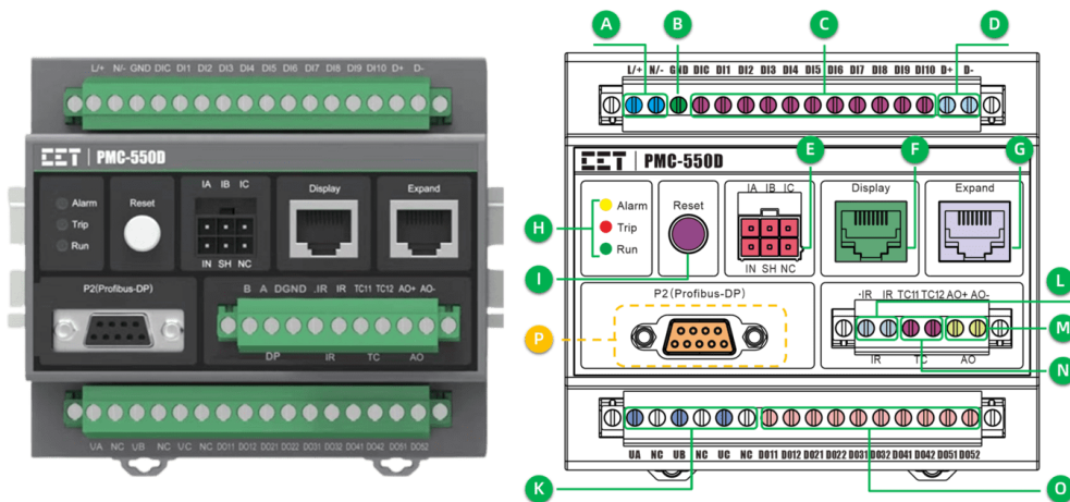
Figure 2-2 PMC-550D Front View and Terminals Diagram (10xDI+1xRS-485+1xProfibus DP+1xIR+1xTC+1xAO+5xDO)
