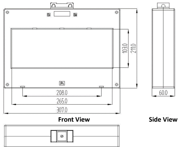
Figure 2-22 PMC-MIR-265 Dimensions
