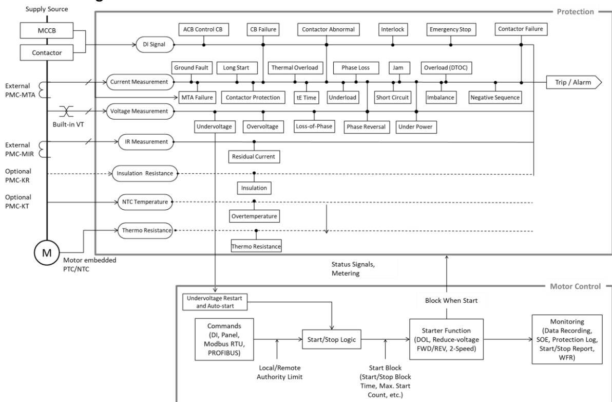
Figure 1-1 PMC-550D's Function Diagram
