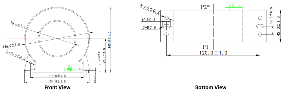
Figure 2-17 PMC-MTA-800A-T Dimensions
