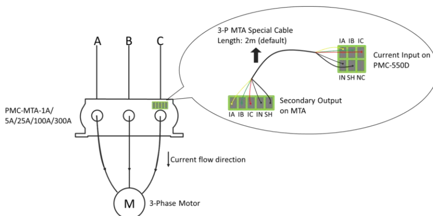
Figure 2-29 PMC-MTA-1A/5A/25A/100A/300A Connections
