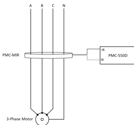
Figure 2-32 Residual Current Input Connection
