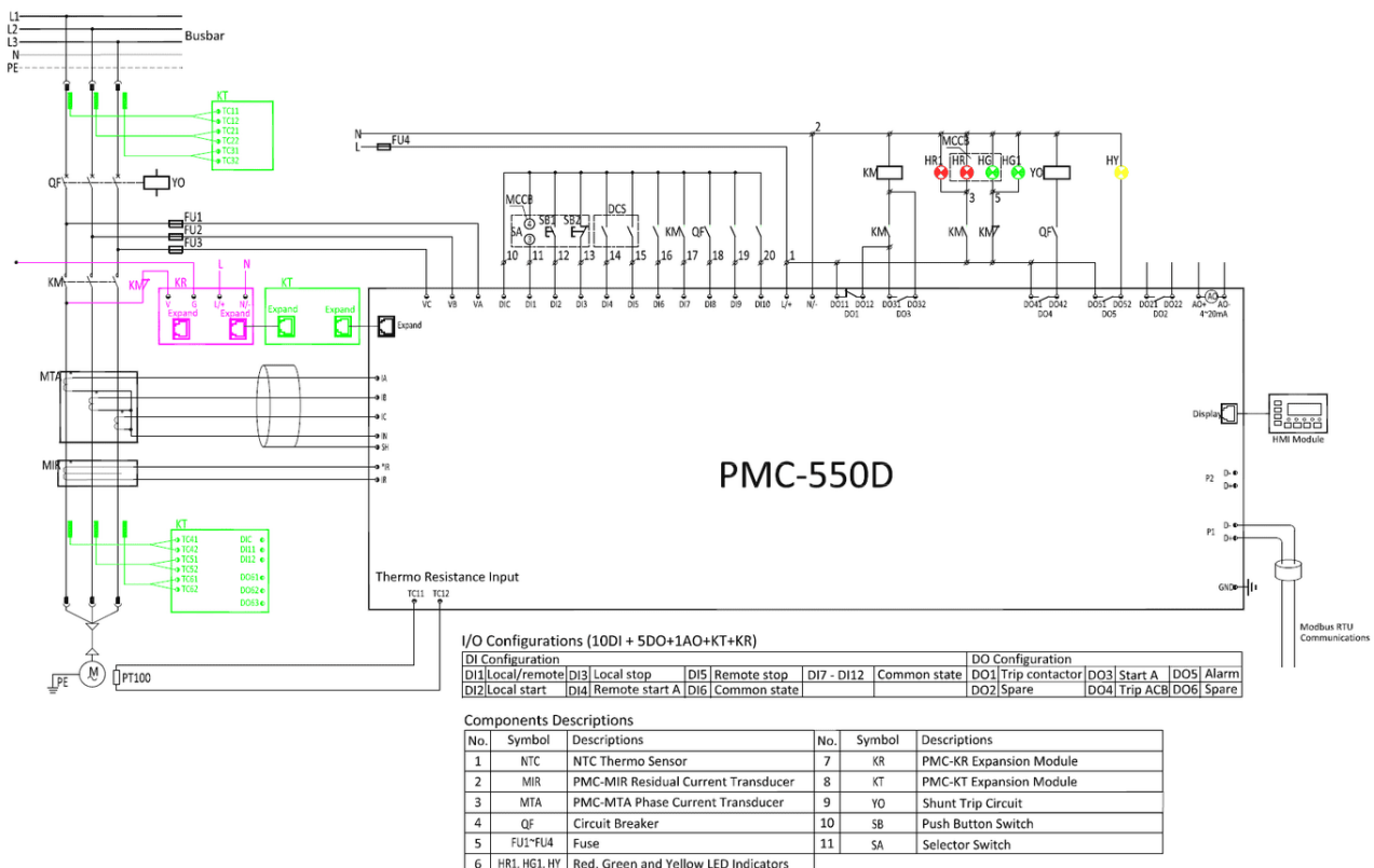
Figure 2-37 DOL Start Schematic Diagram
