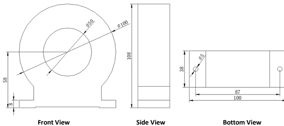
Figure 2-19 PMC-MIR-50 Dimensions
