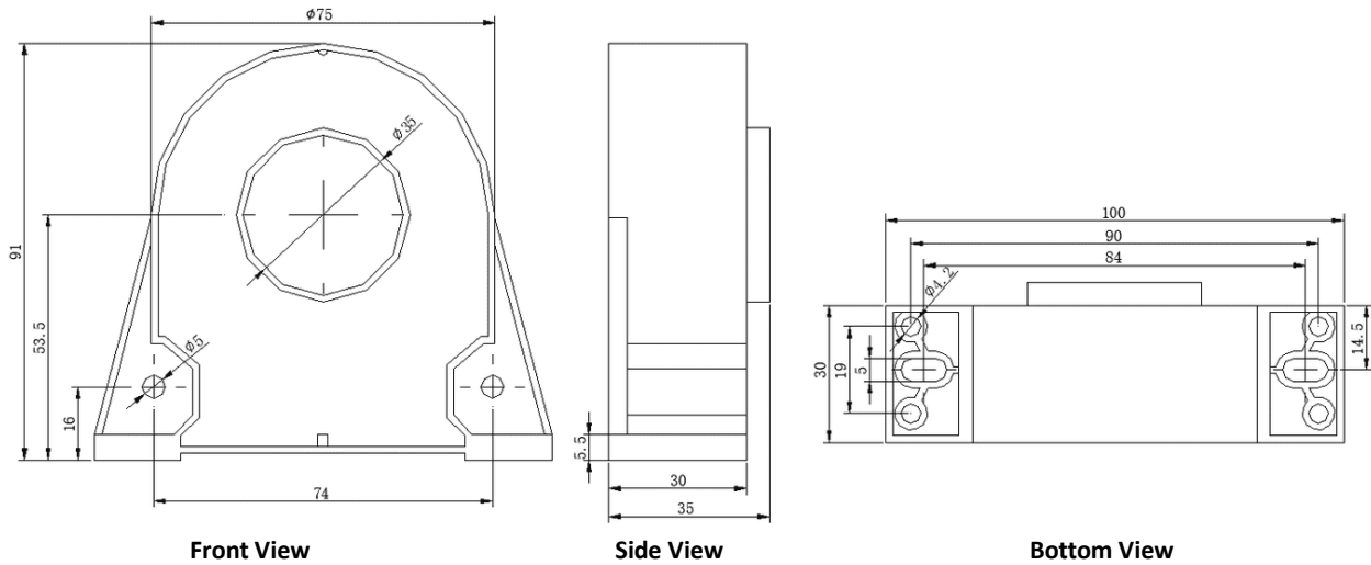
Figure 2-18 PMC-MIR-35 Dimensions
