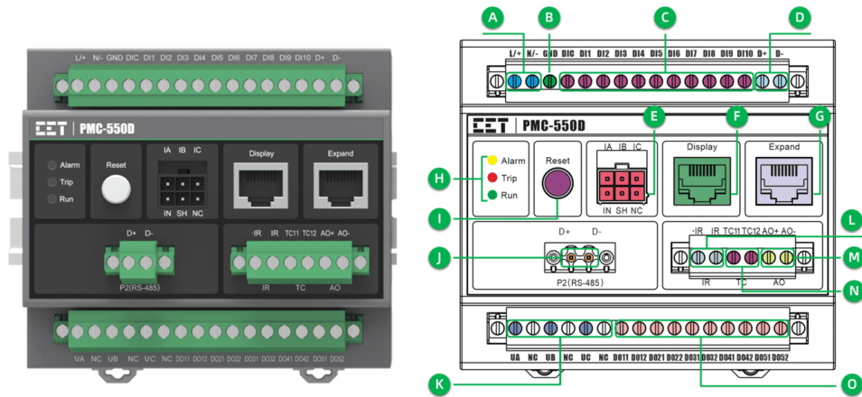
Figure 2-1 PMC-550D Front View and Terminals Diagram (10xDI+2xRS-485+1xIR+1xTC+1xAO+5xDO)
