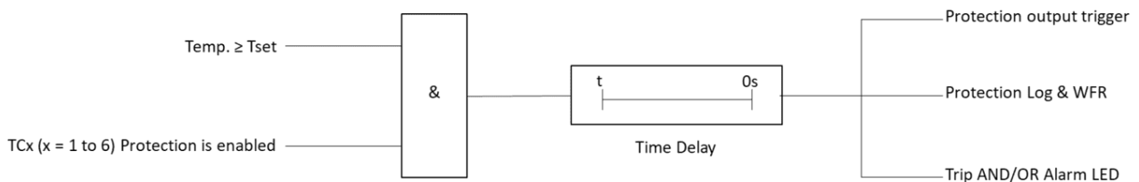
Figure 4-29 Logical Diagram of Overtemperature Protection
