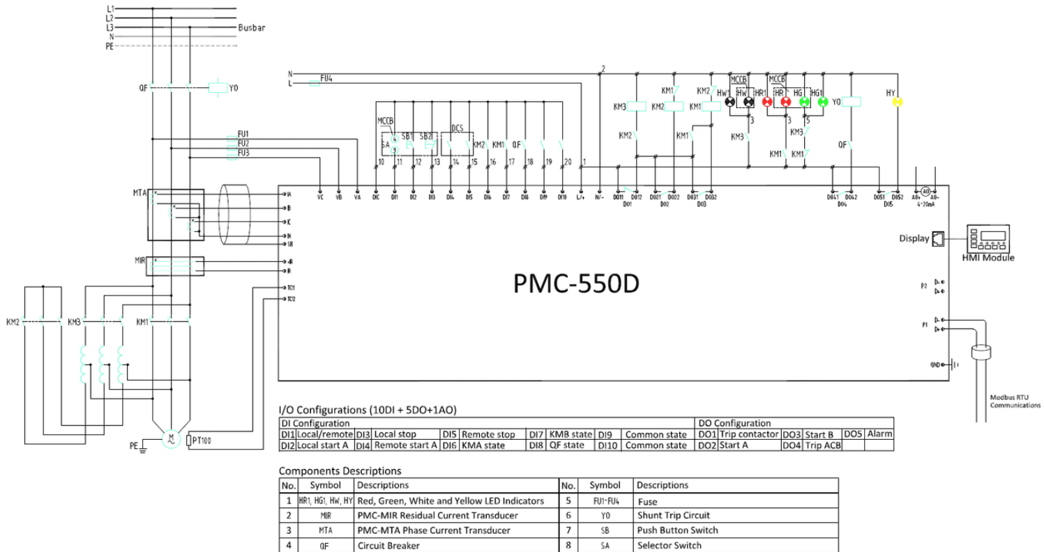
Figure 2-39 Auto-Transformer Operation Schematic Diagram
