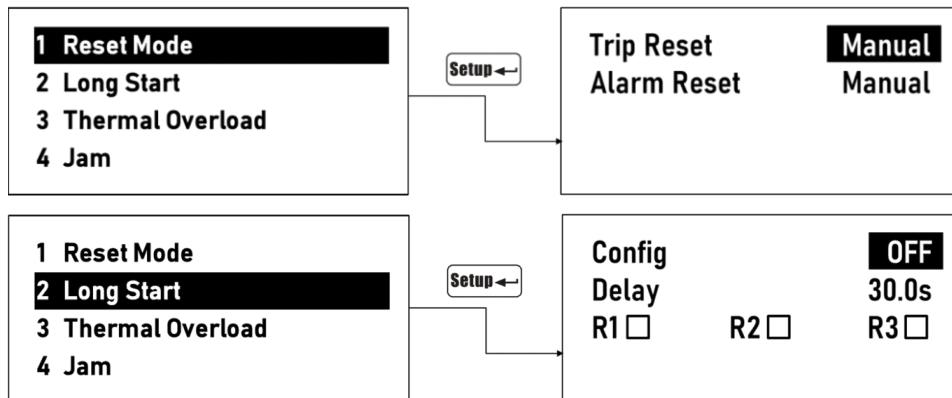
Figure 3-22 Protection Setup Screens
