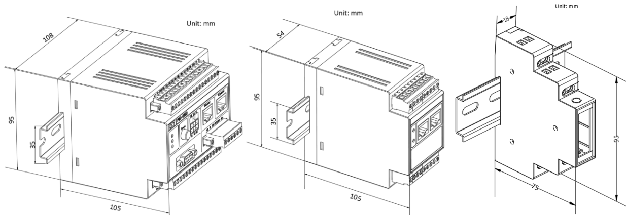
Figure 2-26 DIN Rail Installation for Relay/Expansion Module
