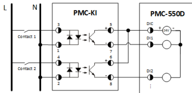
Figure 2-31 Digital Input Connection with PMC-KI Converter
