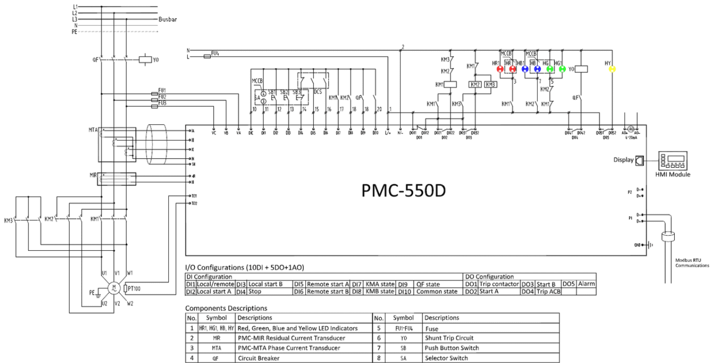
Figure 2-42 Two-speed Operation Schematic Diagram
