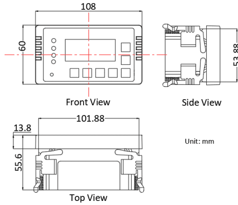
Figure 2-11 HMI Module's Dimensions
