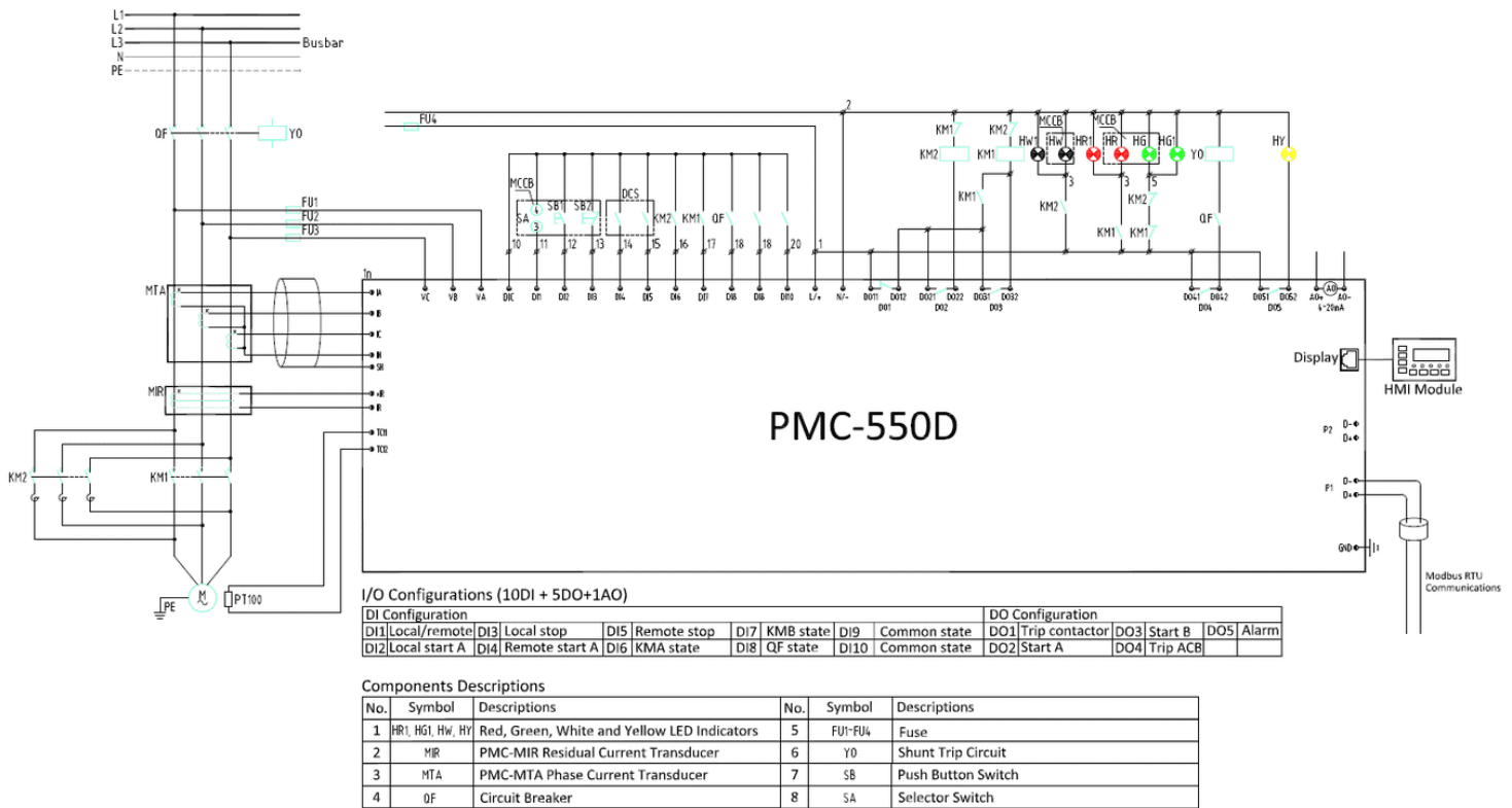
Figure 2-40 Resistance Start Operation Schematic Diagram
