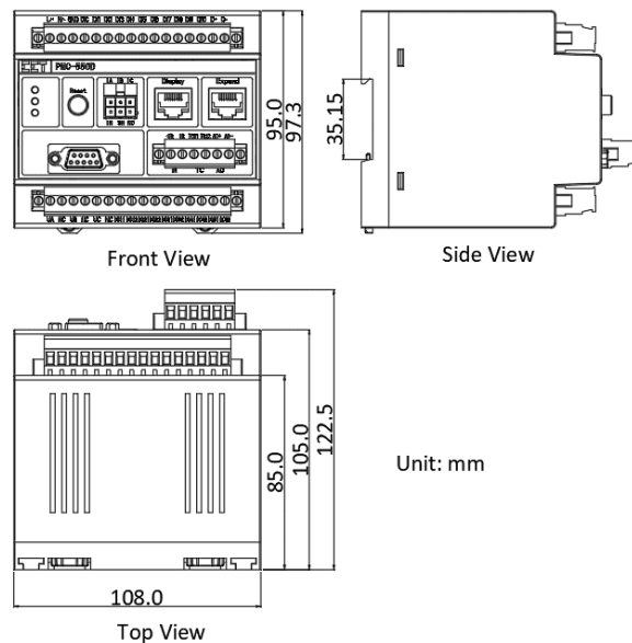
Figure 2-10 Relay's Dimensions
