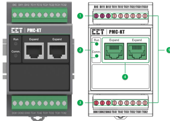
Figure 2-4 PMC-KT Front View and Terminals Diagram
