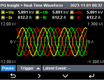
Real-Time Waveform
