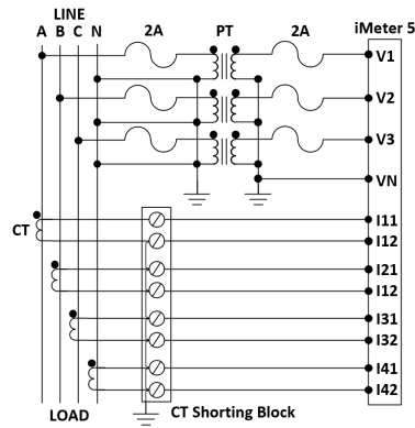
3P4W Wye with 3PTs, 4CTs
