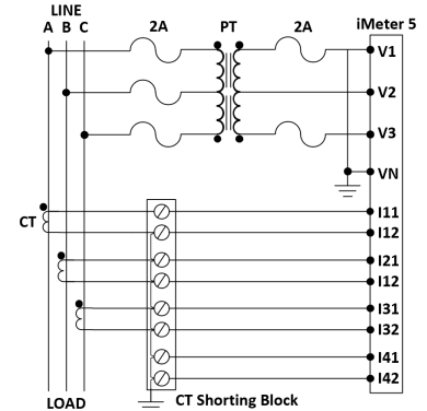
3P3W Delta, 2PTs, 3CTs
