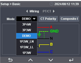
Wiring Setup
