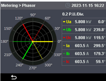
Phasor
