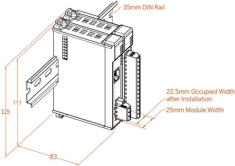
DIN-Rail Installation of Expansion Module
