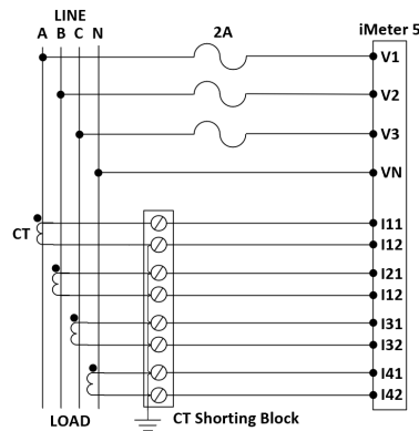
3P4W Wye, no PTs, 4CTs
