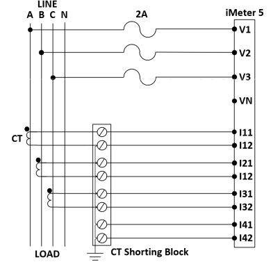
3P3W Delta with no PT, 3CTs
