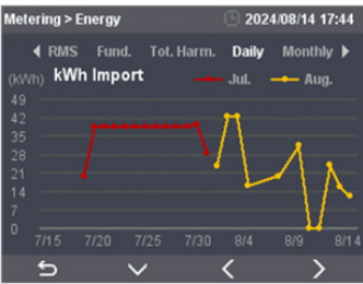
Daily Energy Consum. Curve
