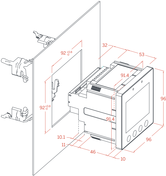
Installation of iMeter 5 Main Unit
