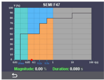
SEMI F47 Curve
