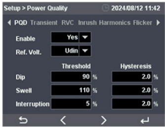
PQ Disturbance Setup
