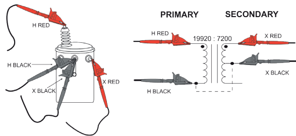
VT/PT Test - Alternate Connection - Ratio 1.383:1
