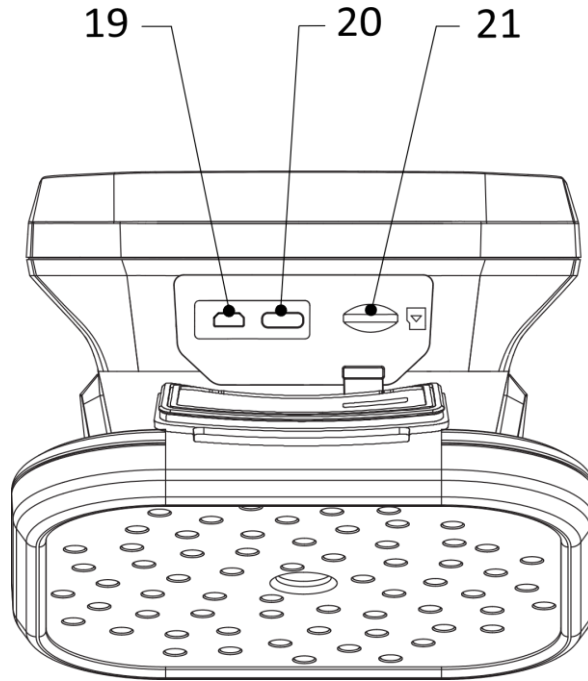
Figure 1-2 USB Interface
