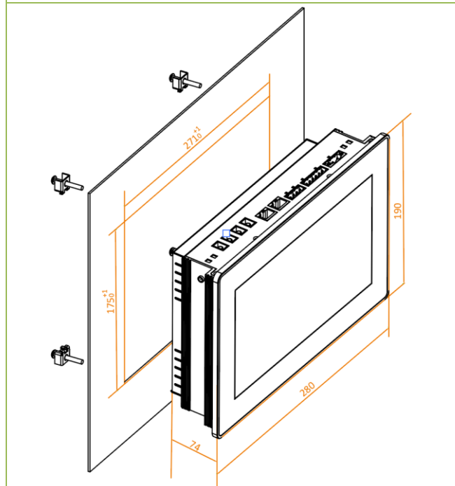
Panel Cutout
