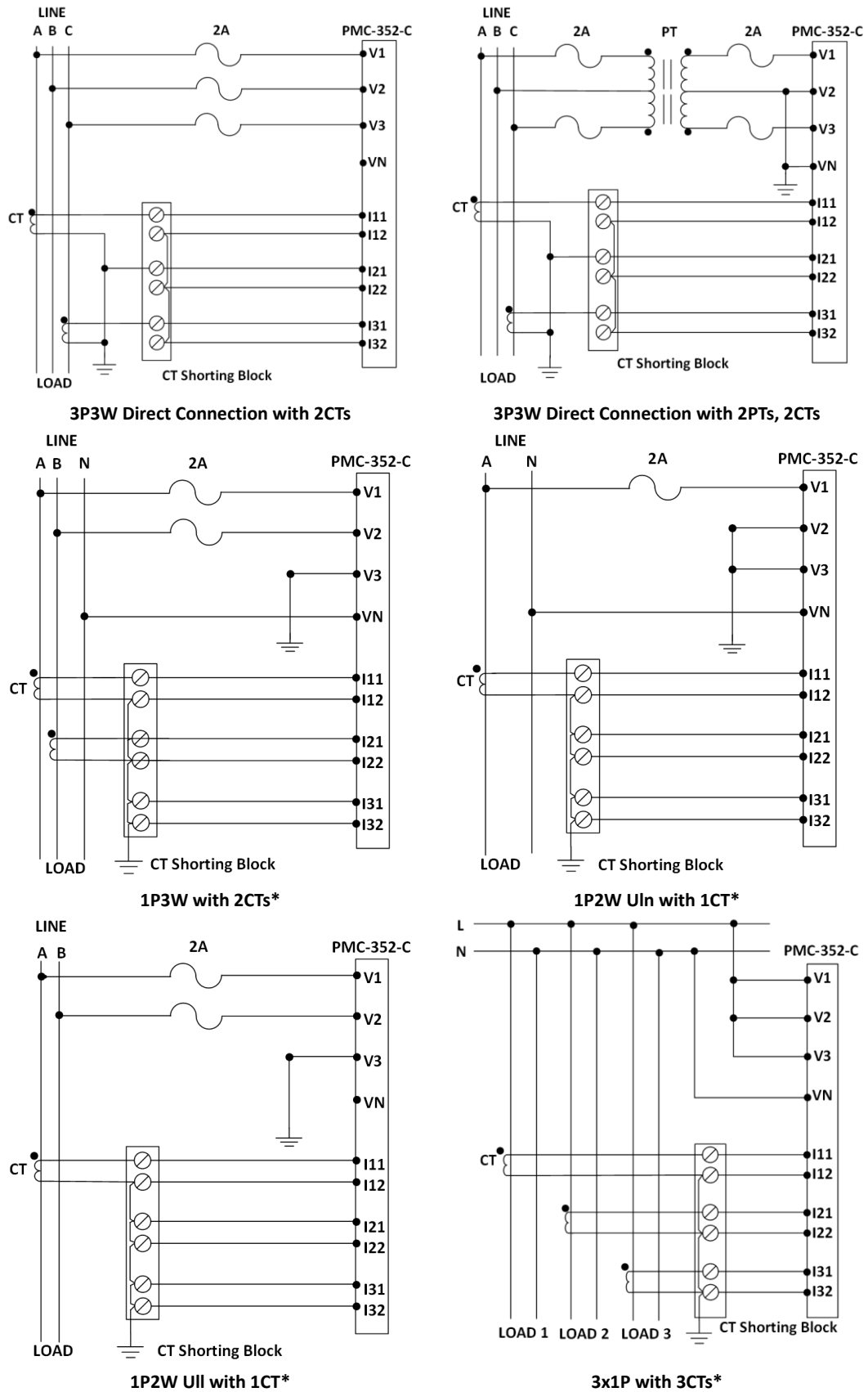
Figure 2-17 Wiring Modes
