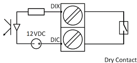
Figure 2-24 DI Connections
