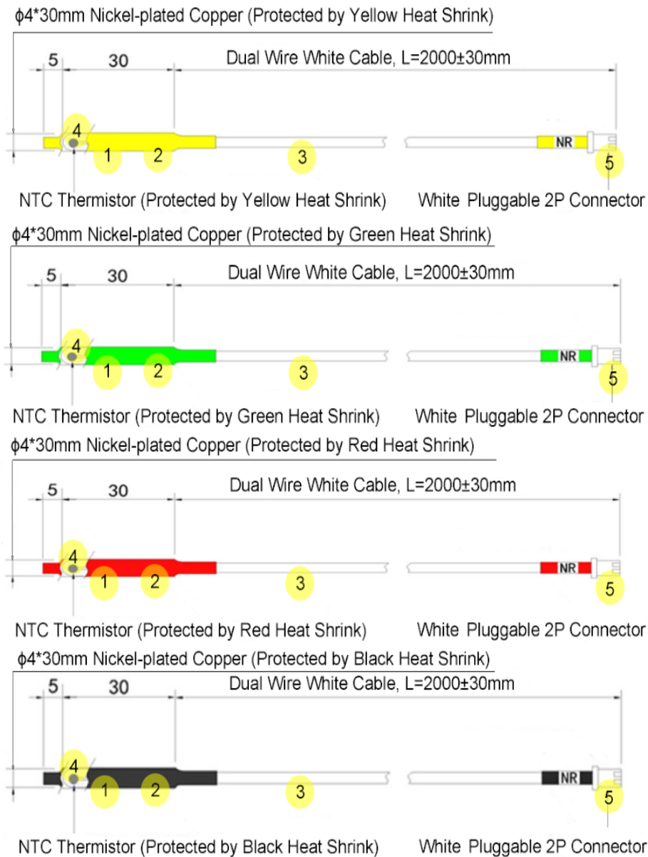
Figure 2-15 NTC-1044, 2 Dimensions
