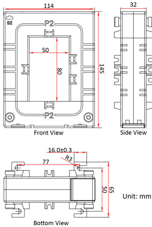
Figure 2-7 800A SCCT Dimension
