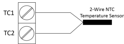
Figure 2-25 NTC Input Connections
