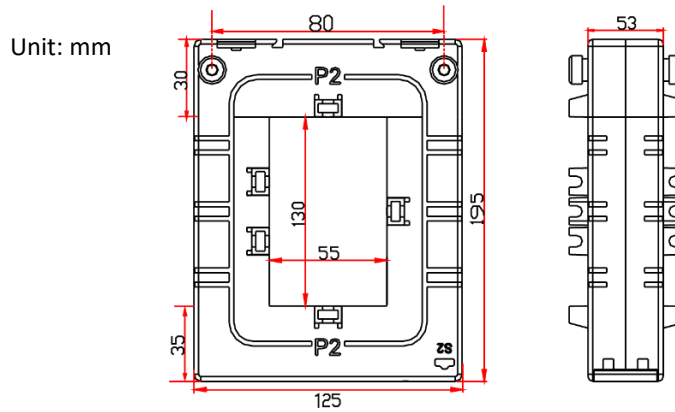
Figure 2-8 1600A SCCT Dimension
