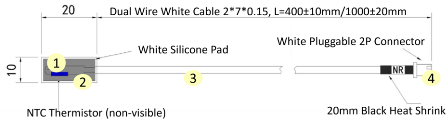
Figure 2-10 NTC-100, 0.4/NTC-100, 1 Dimensions
