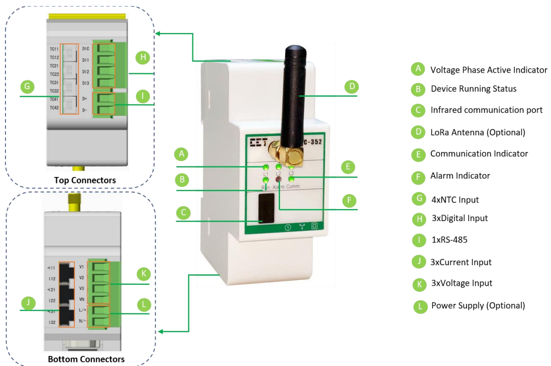
Figure 2-1 Appearance
