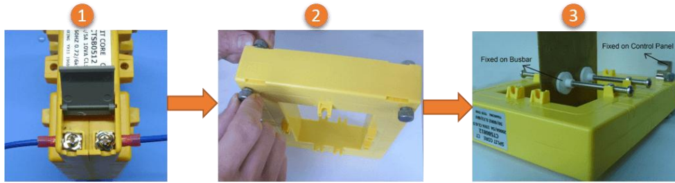
Figure 2-19 800A/40mA, 1600A/40mA SCCT installation
