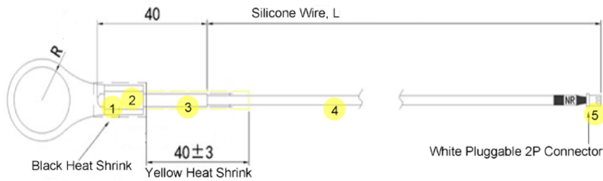
Figure 2-12 NTC-1041, M6, 2/NTC-1041, M10, 1/ NTC-1041, M10, 2 Dimensions
