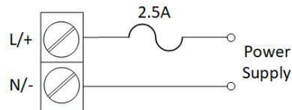
Figure 2-26 Independent Power Supply Connections
