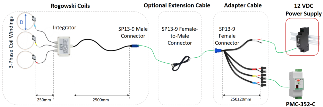
Figure 2-20 Rogowski Coils Wiring
