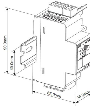
Figure 2-16 Installation
