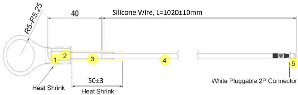
Figure 2-13 NTC-1043, M10, 1/NTC-1044, M10, 1 Dimensions
