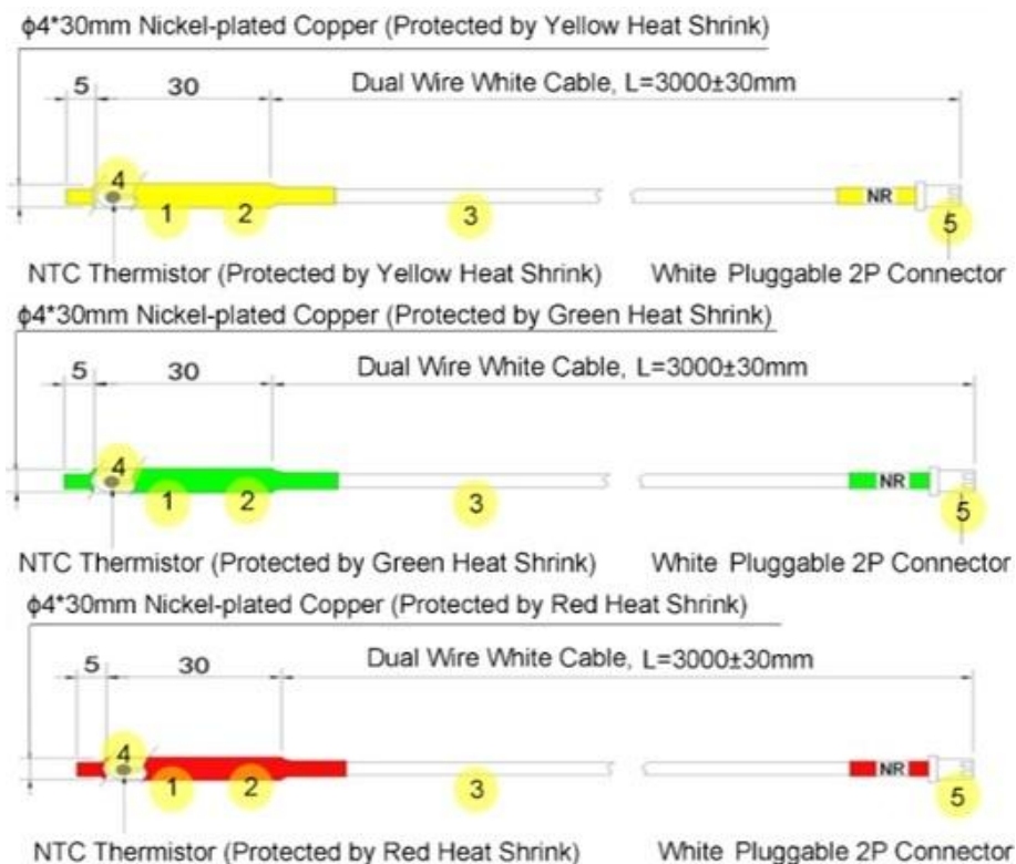
Figure 2-14 NTC-1043, 3 Dimensions
