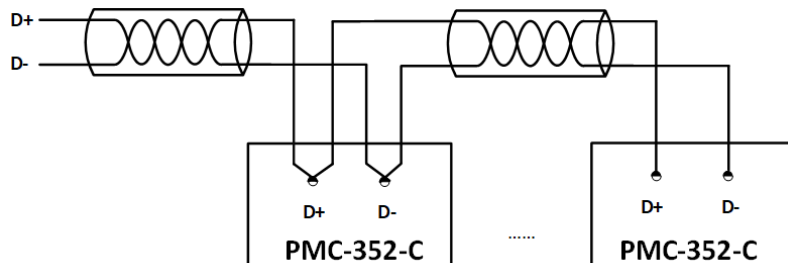
Figure 2-23 RS-485 Connections
