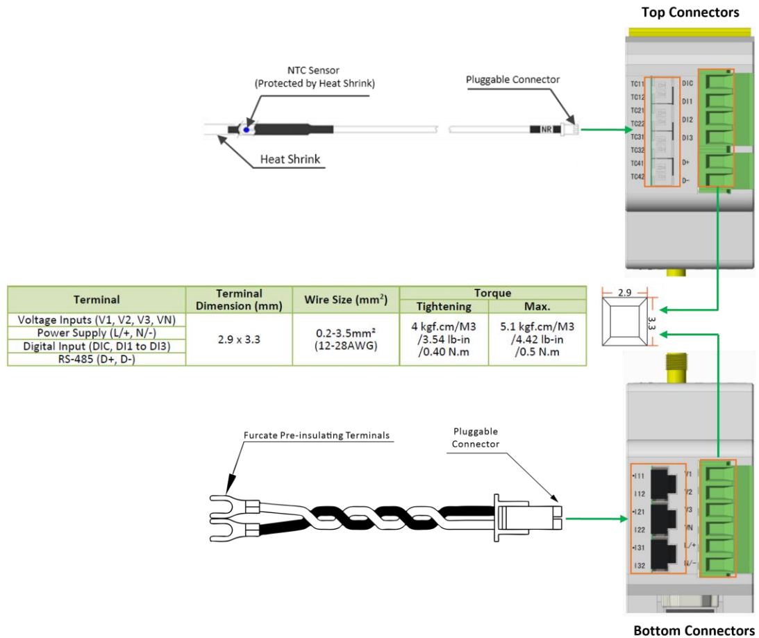
Figure 2-6 Terminal Dimensions
