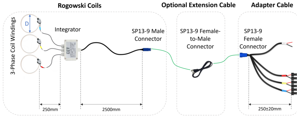
Figure 2-9 Rogowski Coils Dimensions
