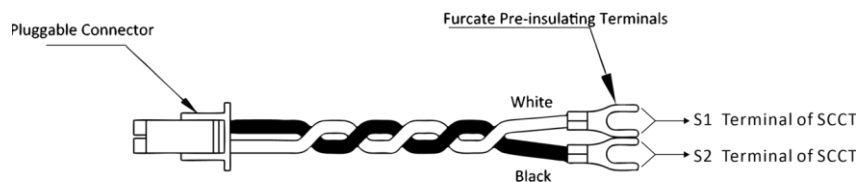
Figure 2-18 5A/2mA, 100A/40mA, 200A/40mA or 400A/40mA SCCT Installation
